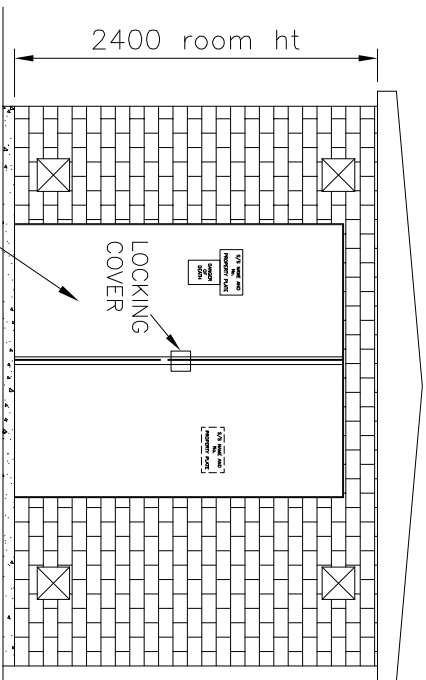
FRONT ELEVATION
